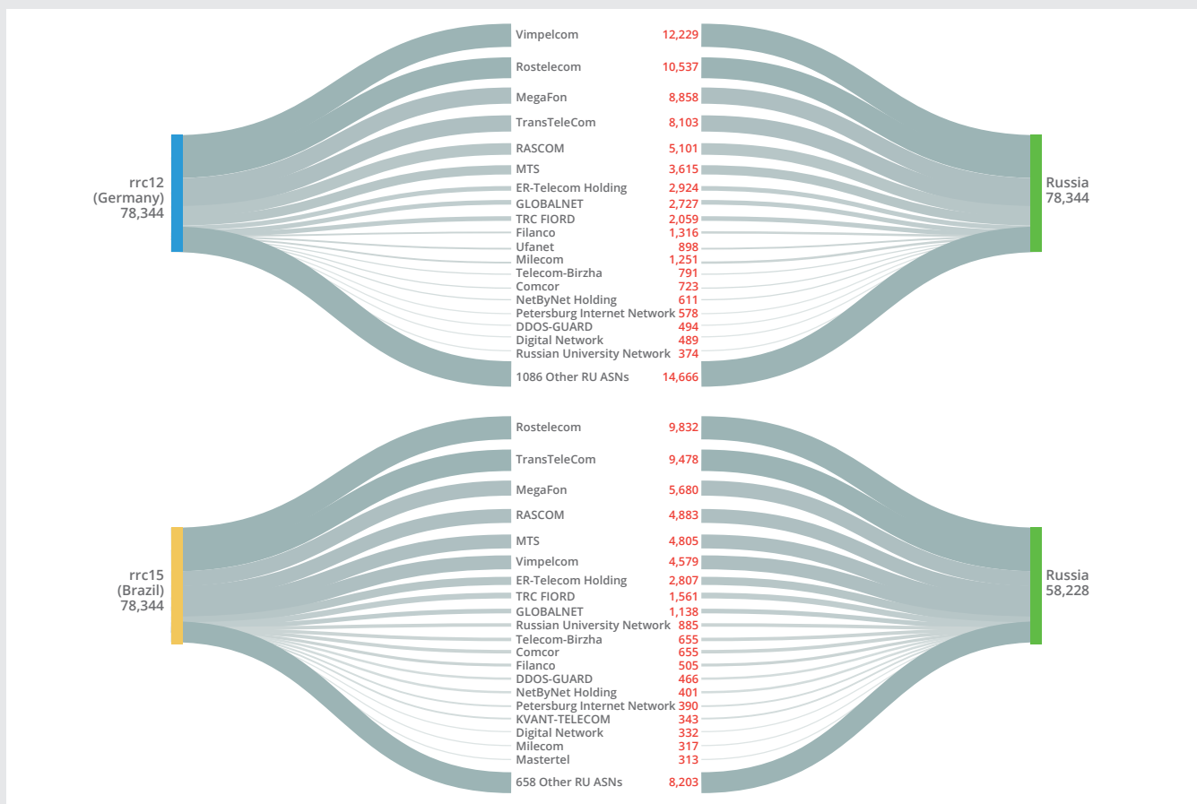
Figure 9: First Russian ASNs observed from Germany (top) and Brazil (bottom), with the number of prefixes passing through each ASN labelled.
