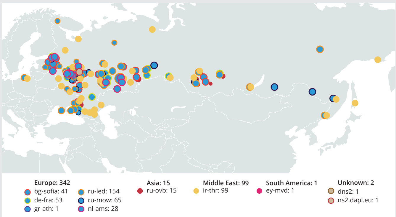
Figure 11: A view of which K-root server answers queries from locations within Russia and Moscow. Different colours represent the continent on which the K-root server is located: blue indicates locations in Europe, yellow the Middle East, and red Asia. The size of each data point reflects the time it took the server to answer the query.
