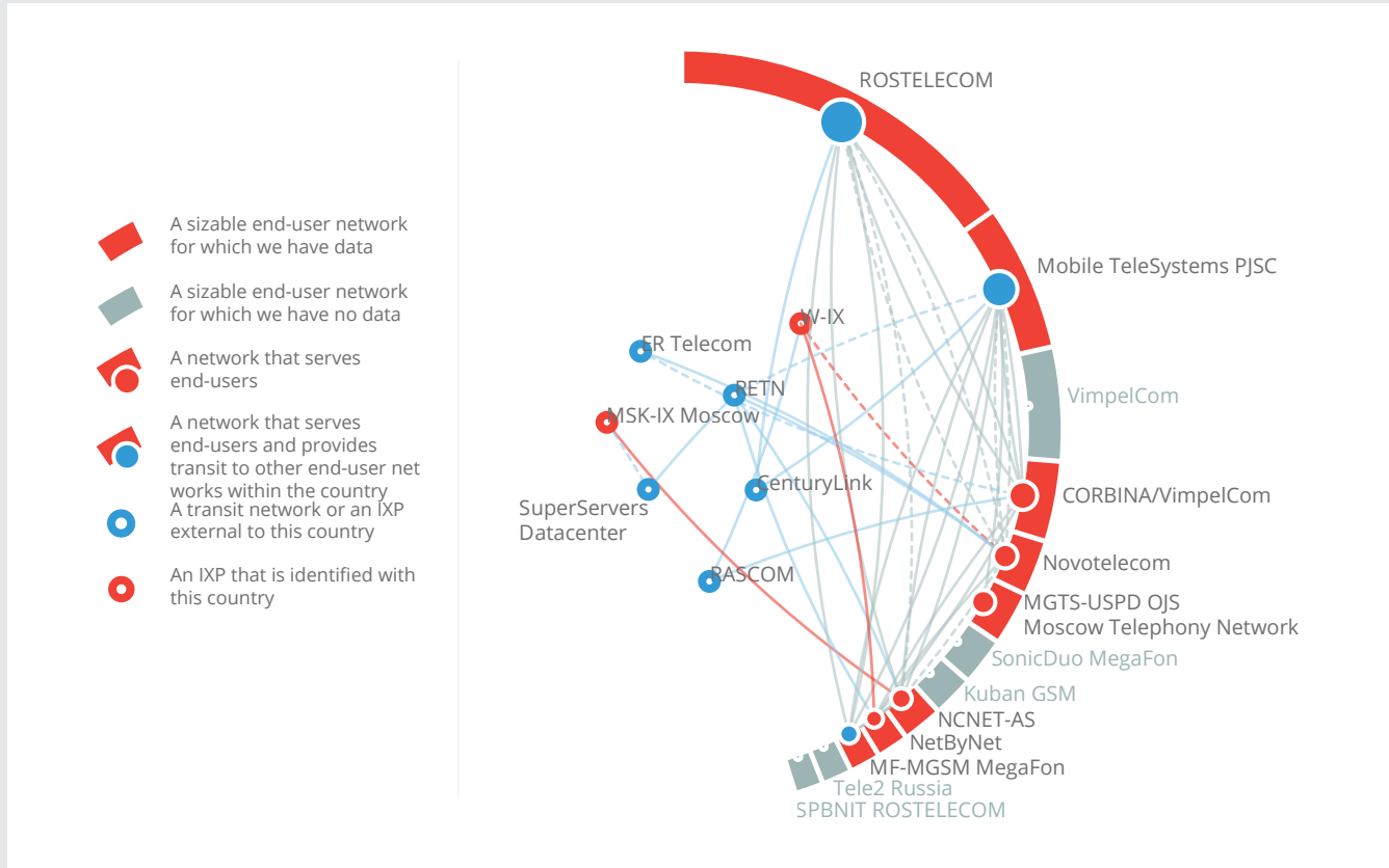
Figure 8: A snapshot of Russian ASNs and the interconnections between them during January 2019. ASNs that are not visible are those that cover less than 1% of Internet users in Russia.
