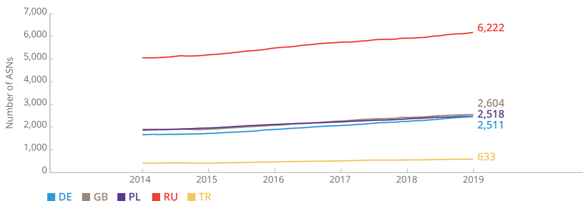
Figure 7: AS Number growth in the last five years.
