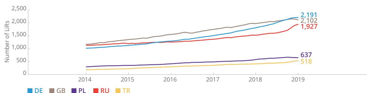
Figure 3: Growth in the number of LIR accounts registered in Russia and other selected countries from January 2014 to January 2019.
